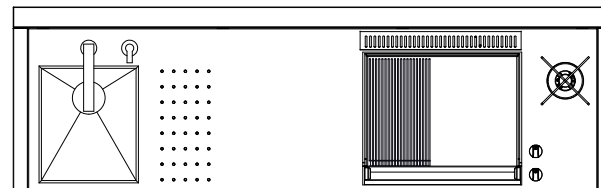
IN 55 Combi LR / Dimensioni piastra - Dimensions Plaque Plate's Dimensions - Platte Abmessungen: 53 cm x 40 cm
