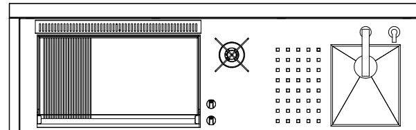
IN 80 Combi LR / Dimensioni piastra - Dimensions Plaque Plate's Dimensions - Platte Abmessungen: 79 cm x 40 cm
