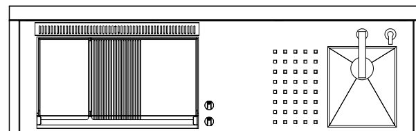
IN 80 MIX LR / Dimensioni piastra - Dimensions Plaque Plate's Dimensions - Platte Abmessungen: 26+53 cm x 40 cm
